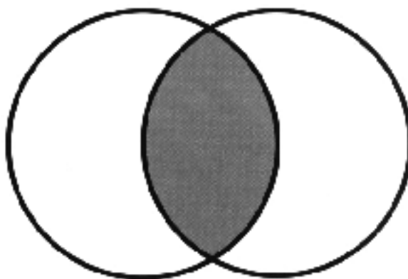
The area of the Vesica Piscis
